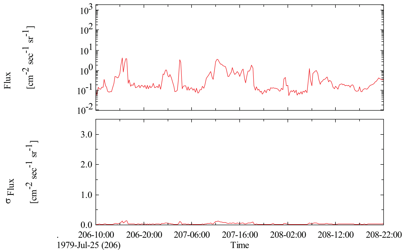
Voyager 2 CRS Proton Flux (1.8-8.1 MeV) from L[1][2][4] at Jupiter, Low Energy Telescope
